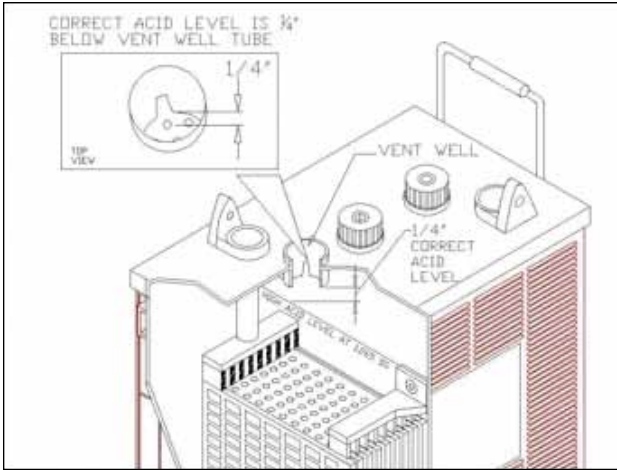
Figure 4 – Electrolyte level
