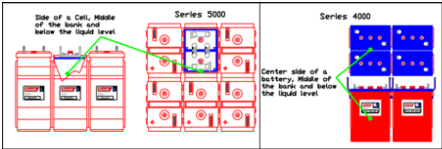
Figure 5 – Temperature Probe
